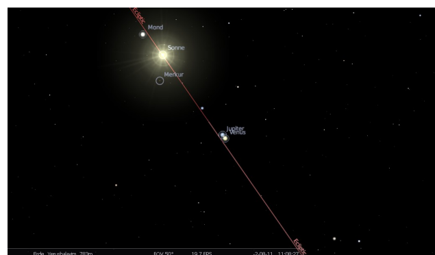
Figure 6: Venus and Jupiter one day before conjunction
